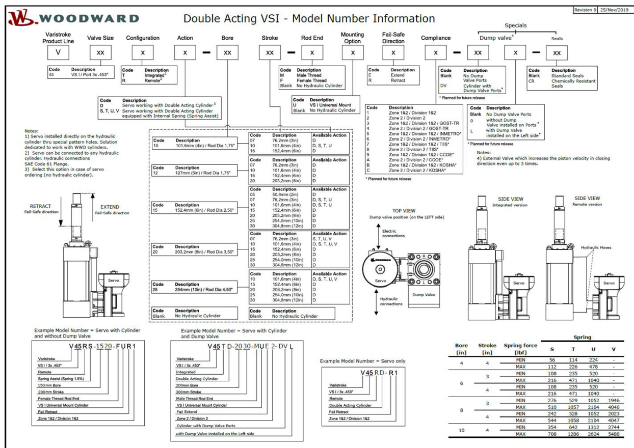
Figure 5-1. Double Acting VariStroke I Model Number Information
